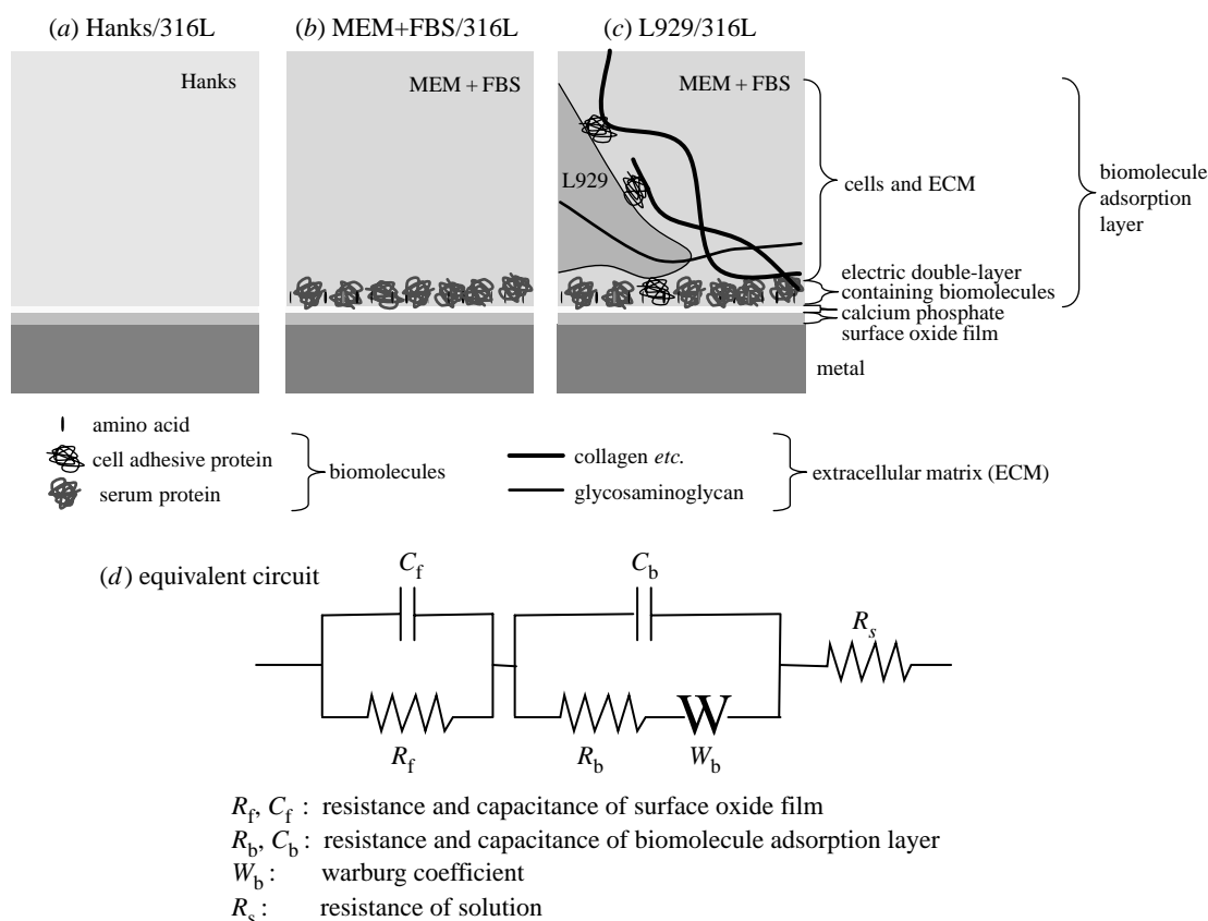
Figure 9. Schematic illustration of the assumed interface on 316L steel prepared in various environments and assumed equivalent electric circuit. (a) Hanks/316L, (b) MEM+FBS/316L, (c) L929/316L and (d) equivalent electric circuit.
